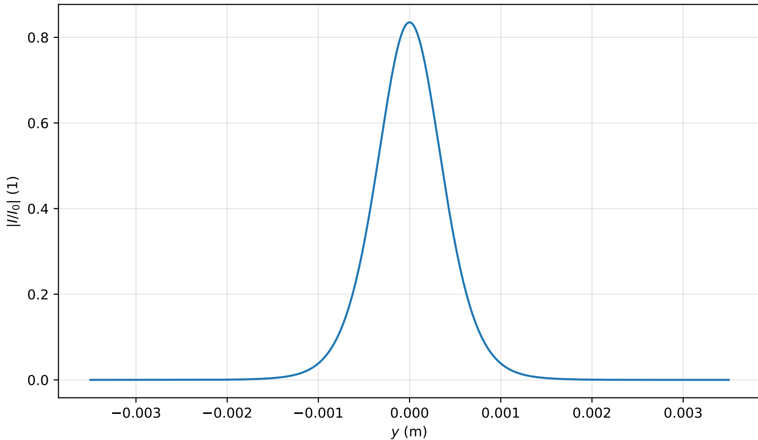
Intensity profile I(x=0, y, z=2.388)/I_0 , P_{in}=0.6P_{cr} , artificial time
